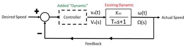
Figure 17: Block Diagram with Controller
