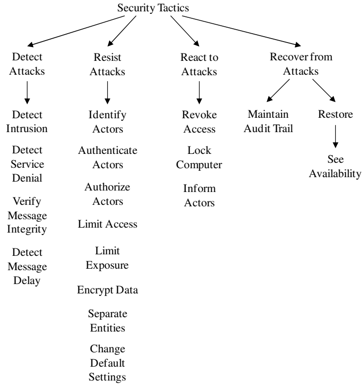
Fig. 4. Classification of security tactics [3].
