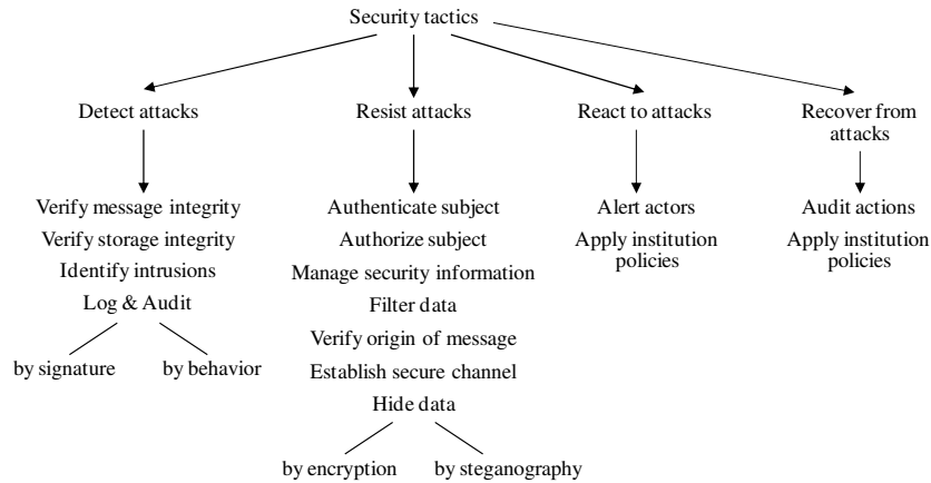
Fig. 5. A new set of tactics.
