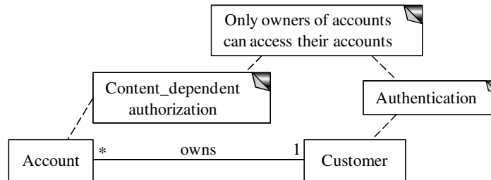
Fig. 3. Hierarchies of policies.
