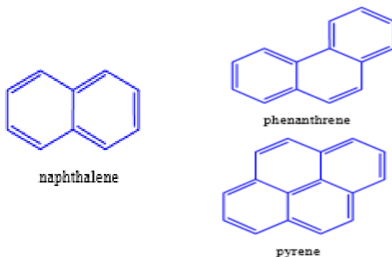
Fig. 1: Molecular structure of the PAHs of interest in this study
